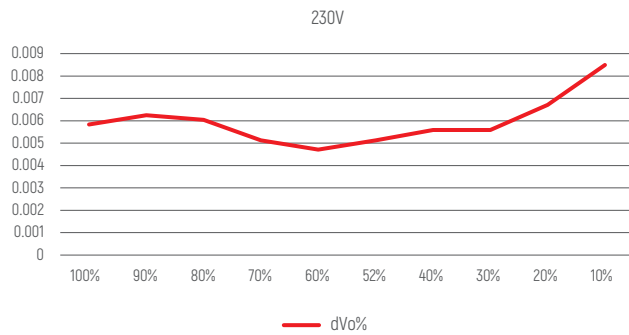
Load adjustment rate curve
