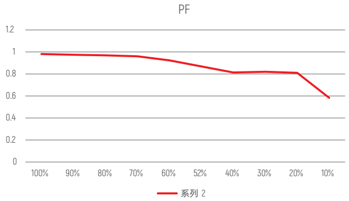
PF VS 负载
