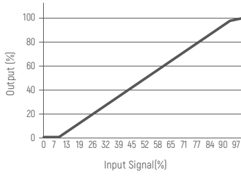
Dimming Curve
